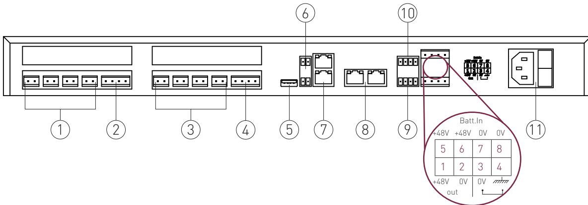
Figure 2 Connection designation of the rear view
