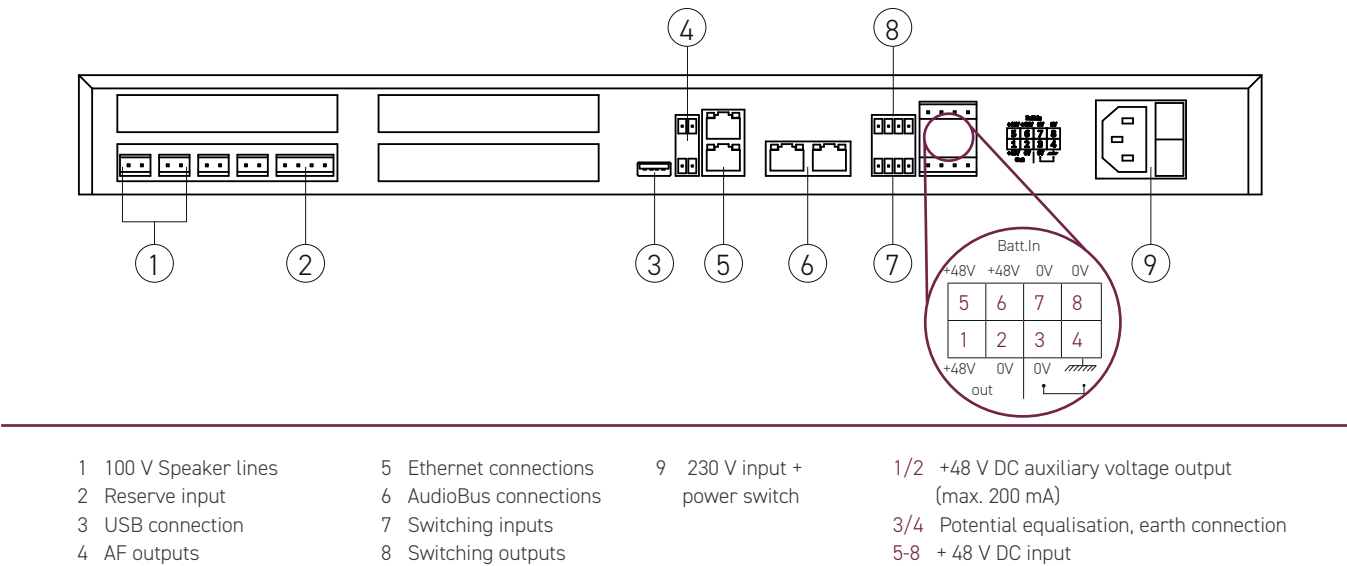
Figure 2 Connection designation of the rear view
