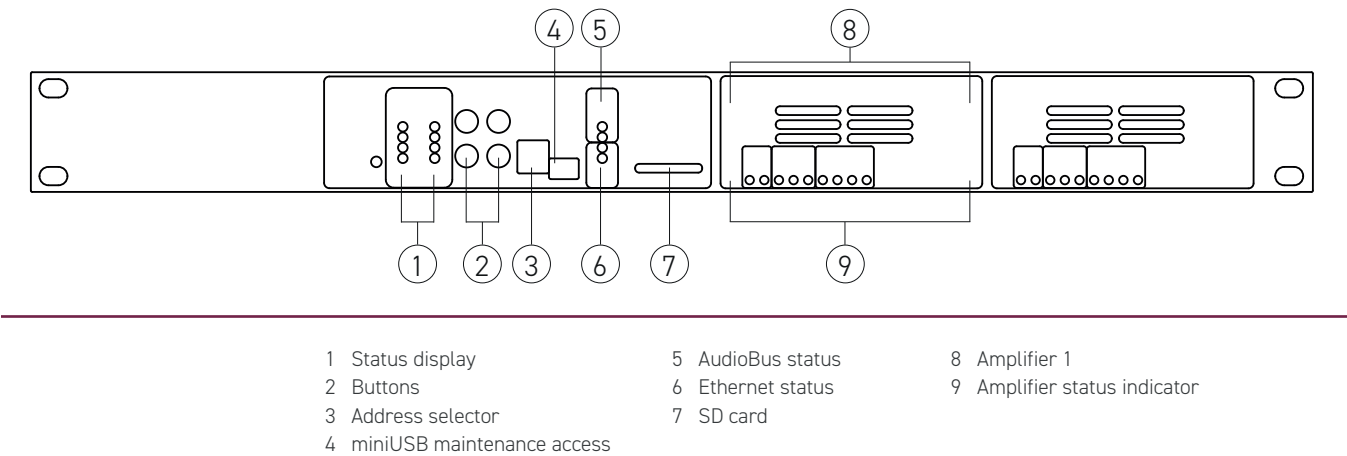
Figure 1 Connection designation of the front view
